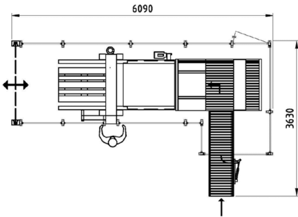
Automatic pallet loader, complex pallet patterns, increased speed
