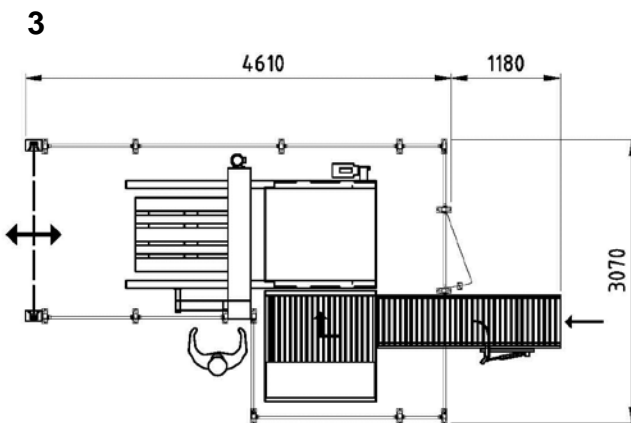
Automatic pallet loader, complex pallet patterns, medium speeds including conveyor with control system and case turn unit
