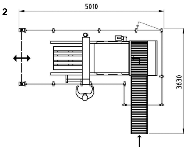
Automatic pallet loader, simple pallet patterns, medium speeds
